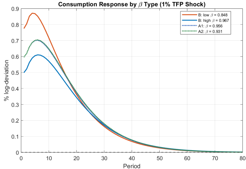
Figure 6: Impulse responses to a one percent TFP shock by \beta types
