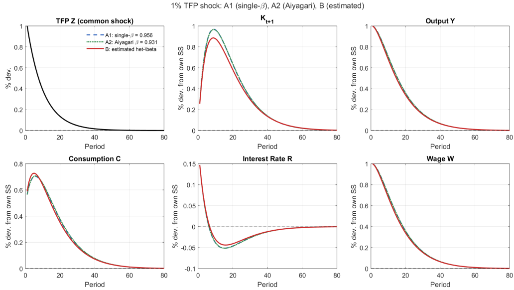
Figure 5: Impulse responses to a one-percent TFP shock across the estimated model and benchmarks
